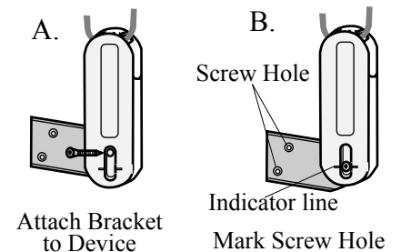
Figure 7. Inside Mount Installation
