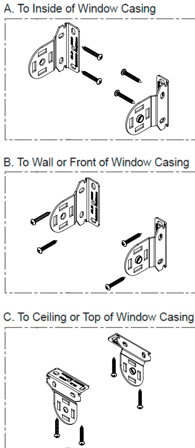
Figure 6. Install Brackets
