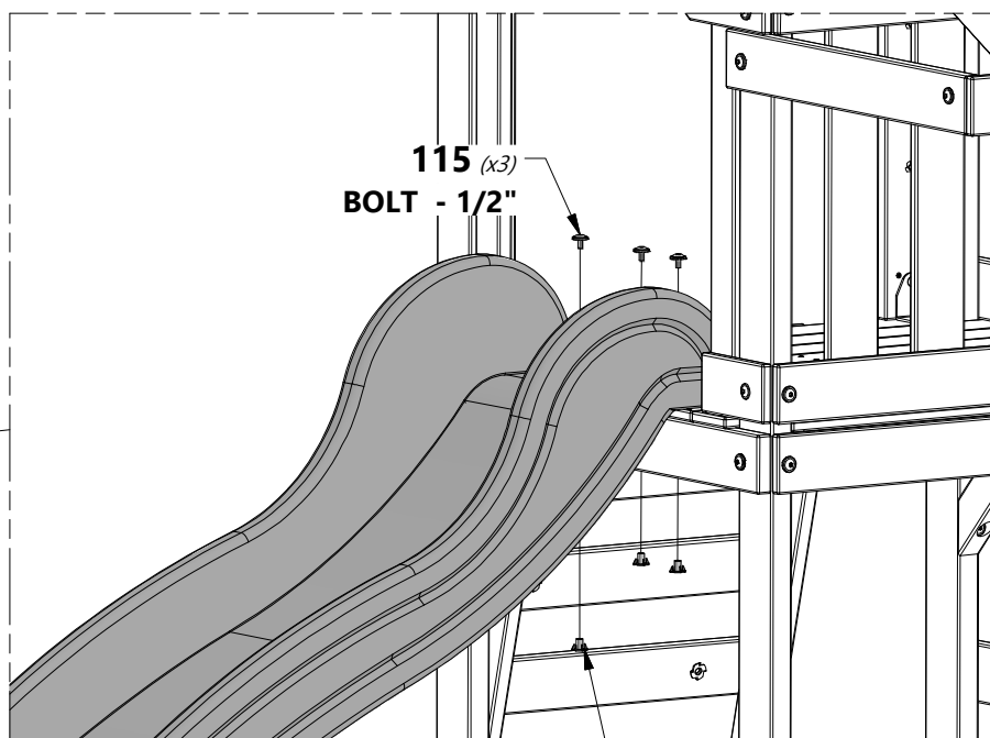
SLIDE BED DRILLING PATTERN
