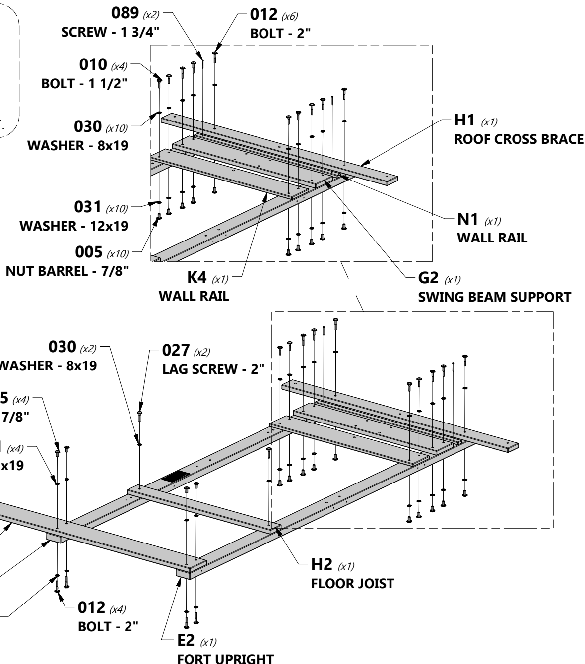
H100089 | SCREW PFH (2) 8x1 3/4
