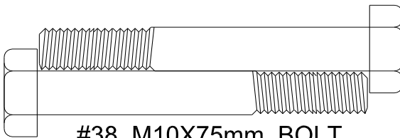
#38 M10X75mm BOLT 2PCS
