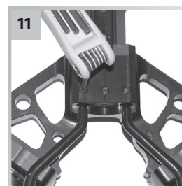
Remove 1/4-inch setscrews holding foot stirrup in place.
