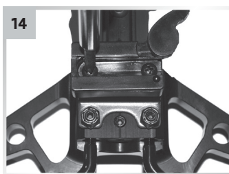
14 Install the quick disconnect (female) attachment.
