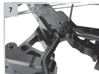
Once the foot stirrup is in place, tighten all three setscrews (if you are not mounting your quiver to the crossbow).
