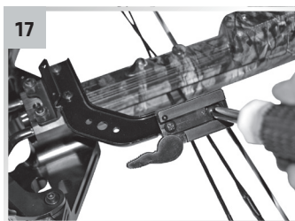
17 Install the female lever-lock attachment.
