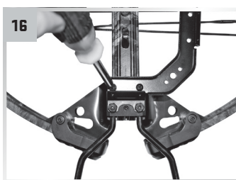
16 Attach the side-mount bracket to the quiver mounting bracket assembly.
