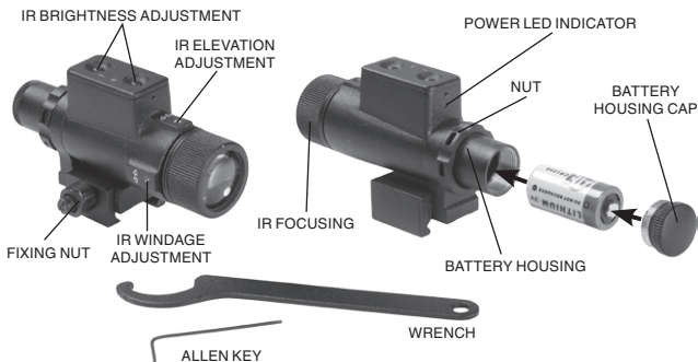
FIGURE 2-8. IR450-B4
