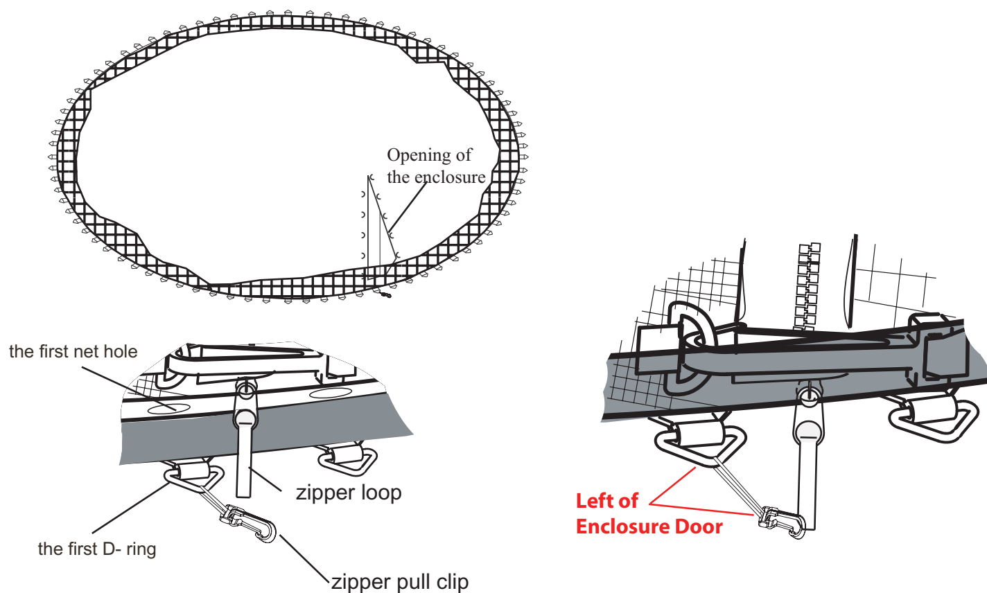
Locked position to secure Enclosure door opening
