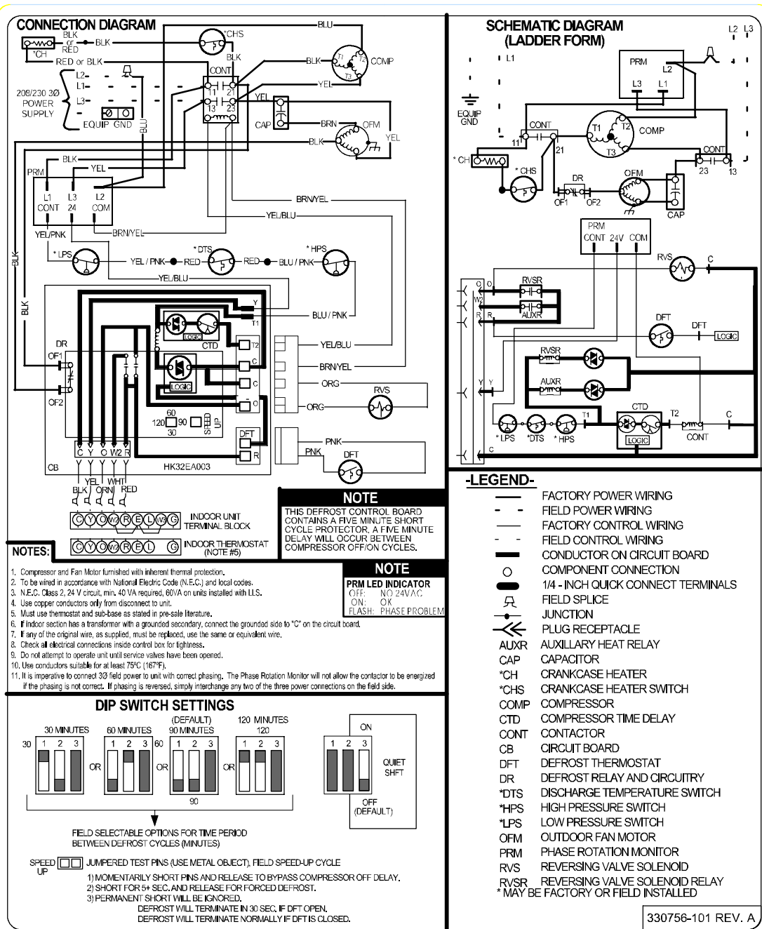
Fig. 3 – Wiring Diagram — Model sizes 030 - 060, 208/230-3
