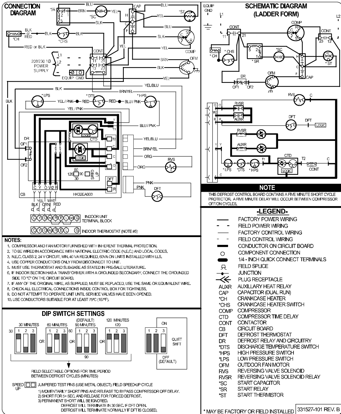
Fig. 2 – Model size 060, 208/230-1
