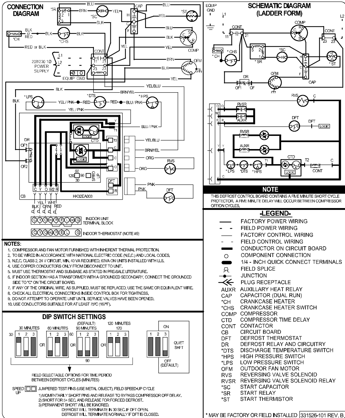
Fig. 1 – Wiring Diagram — Model sizes 018 - 048, 208/230-1
