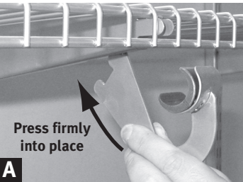
Install rod hanger Install rod hanger into bottom of bracket by tilting it backward until it locks in place. Note: be sure to press rod hangers firmly into place for proper installation.
