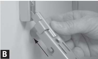
Slide in other end to upright Slide the other end of the upright connector into the bottom two notches of the long upright. Use a level to position the short upright and mark the position of the top & bottom screw holes.
