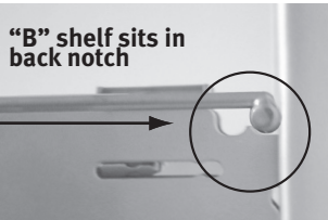
Place shelves onto brackets Shelf labeled "A" sits in front notch of bracket. Shelf labeled "B" sits in back notch. Be sure each shelf slides back as far as possible before locking shelves into brackets. If overlapping three sections of shelving, use two "A" sections and one "B" section, placing "A" sections on the outside and spanning the gap with "B" sections. For four or more overlapping sections, continue alternating between "A" and "B" sections, placing "A" shelves on brackets before "B" shelves.
