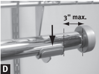
Secure rod and hanger After expanding clothes rod to desired length, place into rod hangers and press down to snap into place. Note: do not extend more than 3" past rod hangers.
