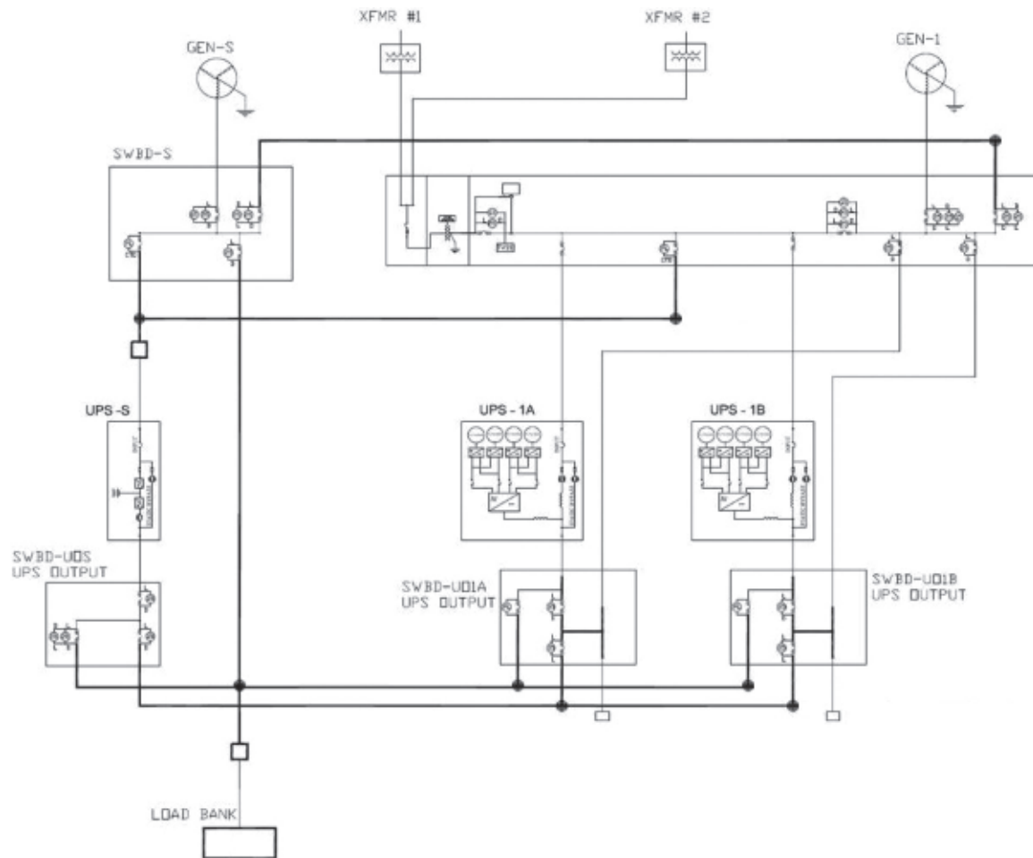
Flywheel UPS & Paralleling Switchgear
