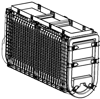
Illustration 5 Assembled air filter
