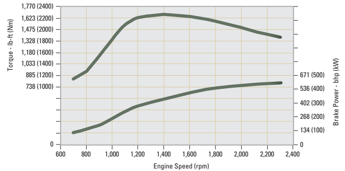
600 bhp (447 kW)
