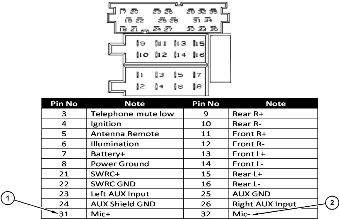
Illustration 4 Radio pin out (1) Mic+ (applies to Bluetooth equipped radios only) (2) Mic- (applies to Bluetooth equipped radios only) g06794044
