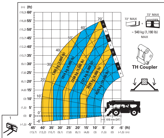
Outriggers Down
