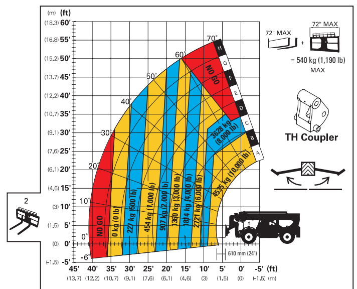
Outriggers Up
