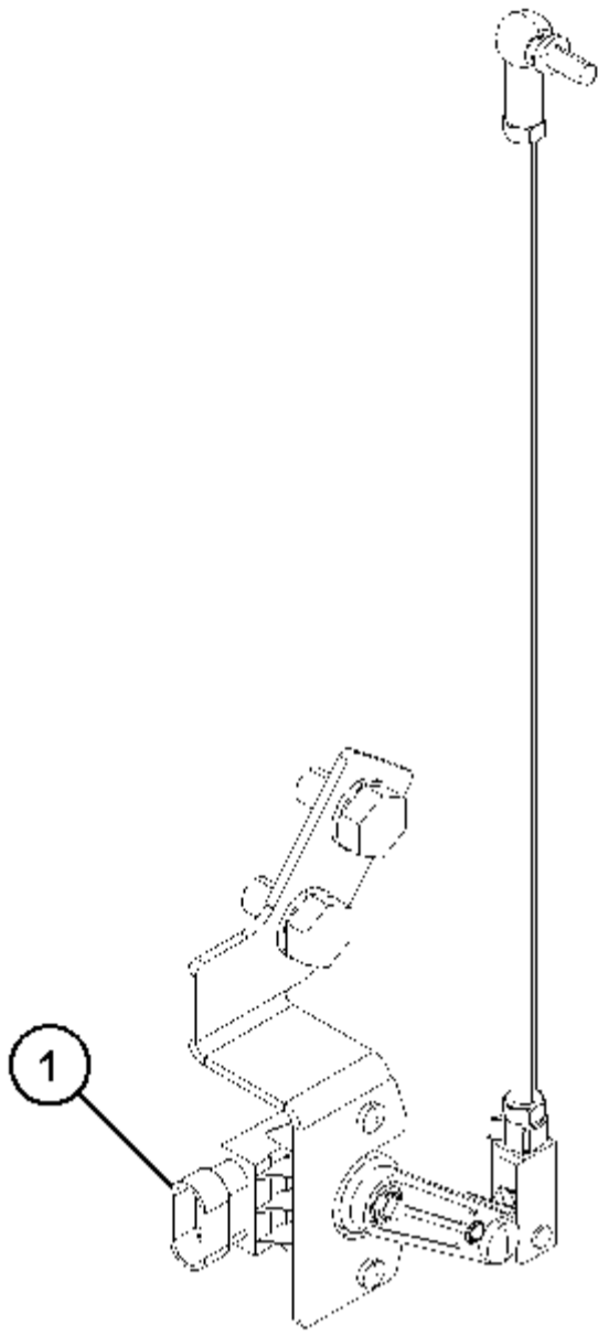
Illustration 2 View of area A Sensor and mounting group Some parts are removed for clarity (1) 621-6556 Angle Sensor
