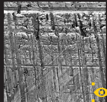
Magnified image of abrasive wear on a piston ring.
