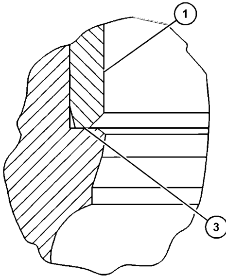
Illustration 8 Typical example Cylinder liner (1) is installed and has complete contact (3) with bottom of cylinder bore g07603913
