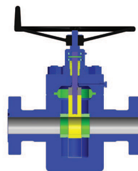
Cut away of valve
