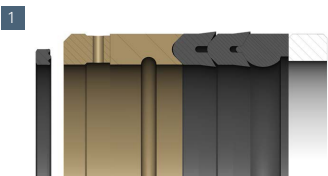
Frac Pump Low Pressure Packing complete set
