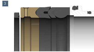
3 Well Service Pump Packing complete set (see below).
