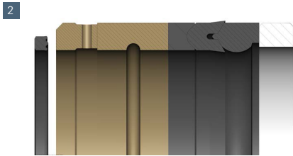
2 Frac Pump High Pressure Packing complete set (above).
