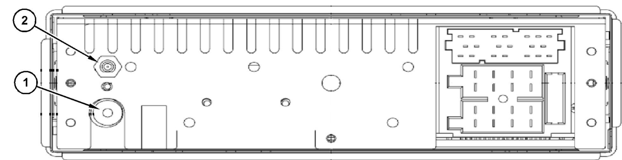
Illustratie 3 g06247910 (1) DAB SMB-connector (2) AM/FM ISO-connector
