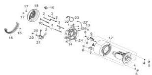
FIG.18 ROTOR/STATOR (F63)
