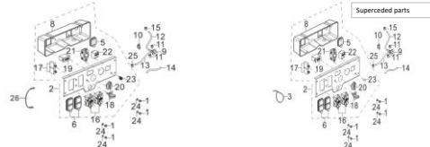
FIG.17 PANEL SUBASSEMBLY, CONTROL (F62)
