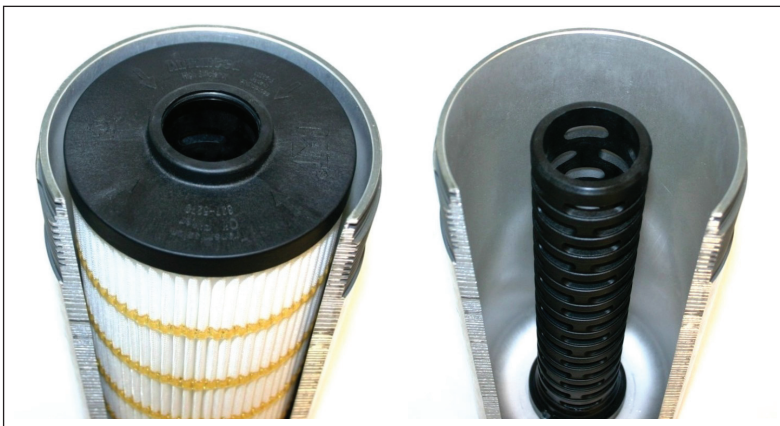
Filter element shown in the filter housing prior to servicing the filter element.
