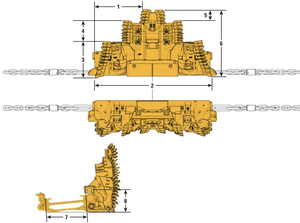
Dimensions – Plow Body Setup Option 3 (All dimensions are approximate.)
