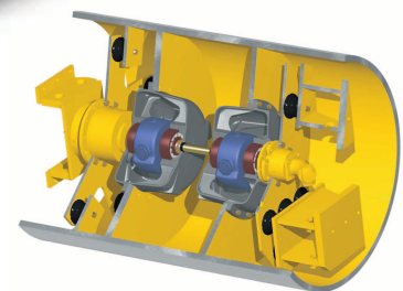
Cat Pod-style Vibratory System
