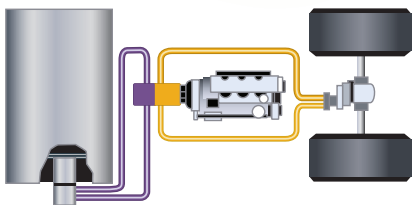
Cat Dual Pump Propel System
