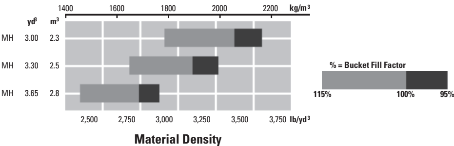
Pin-On Bucket Selection Guide
