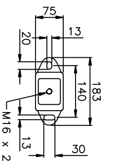
FLEXIBLE ENGINE MOUNT 'B'
