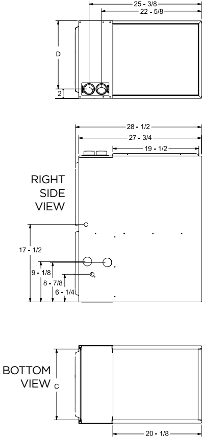
TOP VIEW
