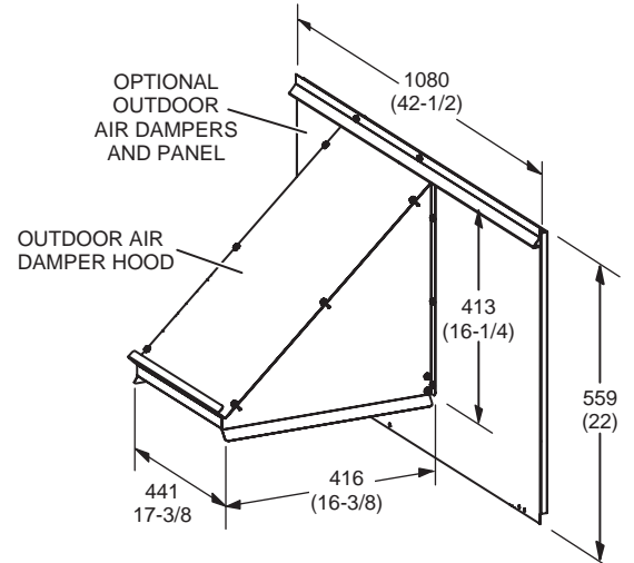
END VIEW
