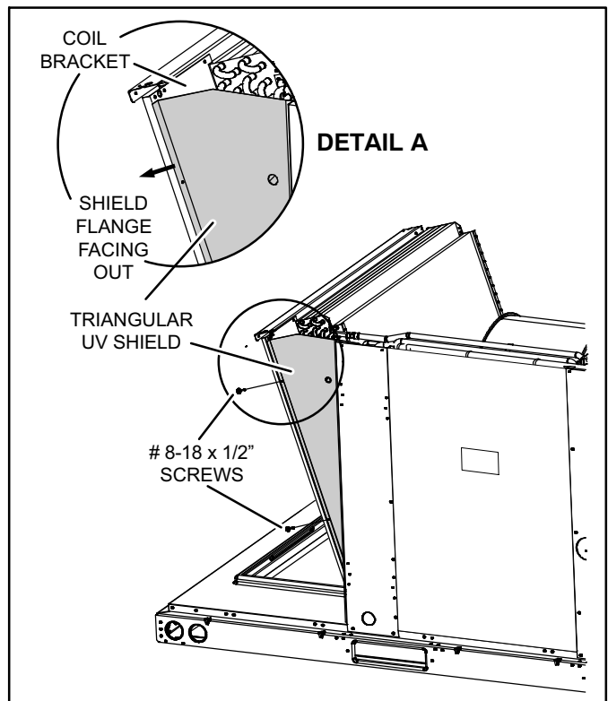
Figure 11. Installing Triangular Panel
