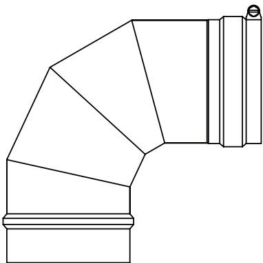
90° ELBOW (Typical)
