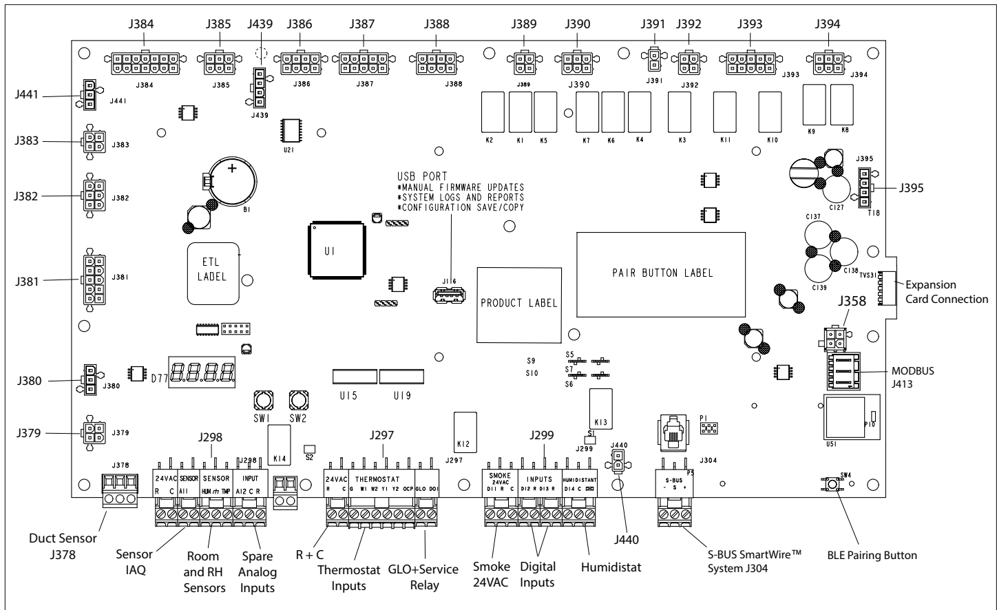
Figure 1. Intelli-Guide™ Unit Controller and Expansion Port Locations
