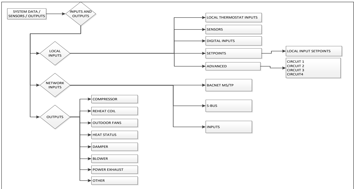
Figure 20. System Data / Sensors / Outputs Menu Structure
