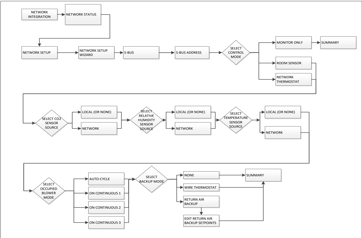
Figure 10. S-BUS Menu Structure
