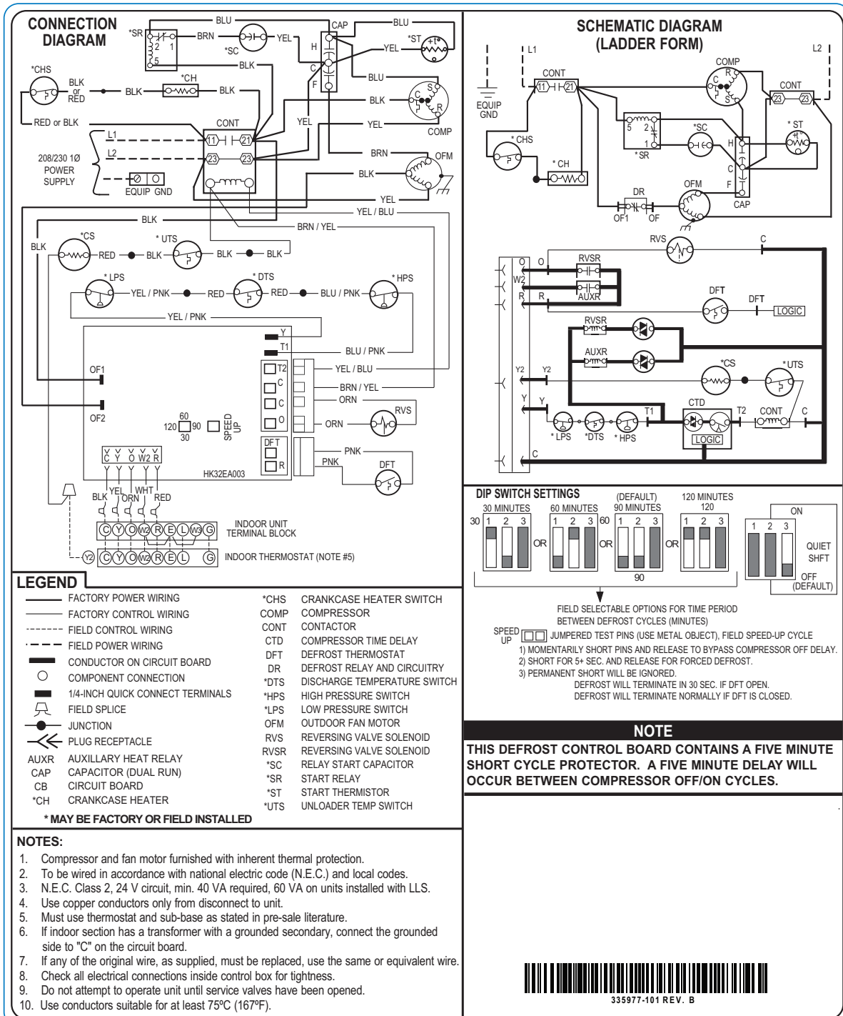
Fig. 1 - PH16NA 2 - 5 Tons
