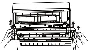
Fig. 13 — Lift the front panel
