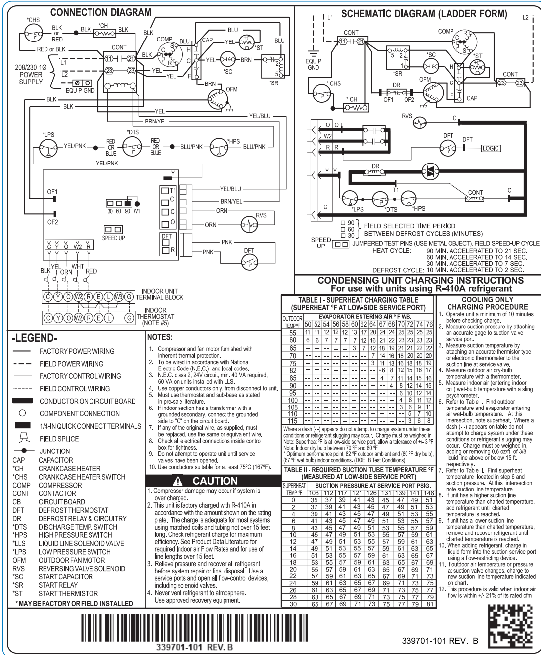
Fig. 1 – Wiring Diagram — Model sizes 1-1/2 - 4 Tons, 208/230-1
