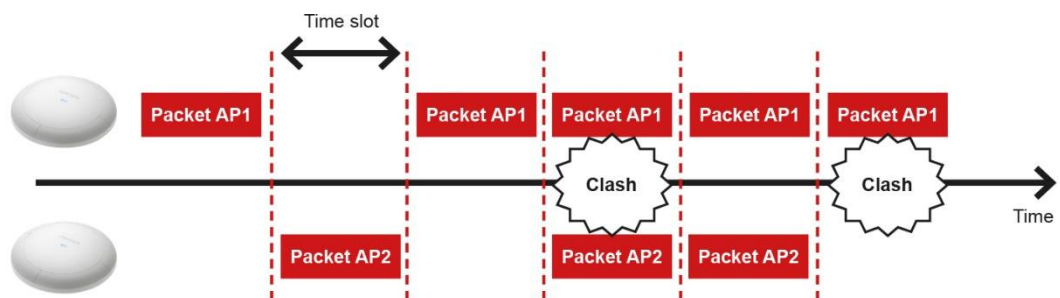
Figure 2-4: Simulation of interference and contention risk with multiple APs
