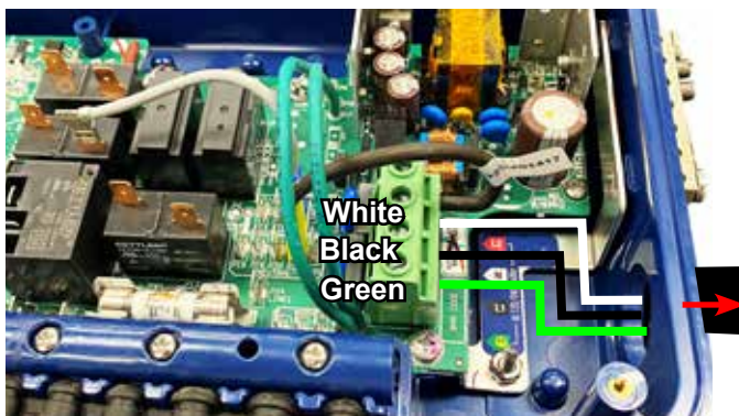
Field Converted 110V 30 AMP Control Box
