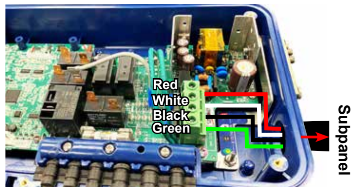
Field Converted 110/230V Control Box
