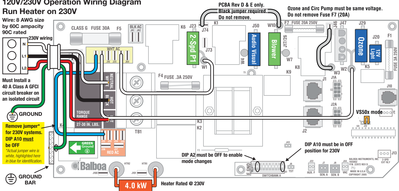
Figure A3. Wiring Diagram for 120V/230V Permanent Wired Option 2.
