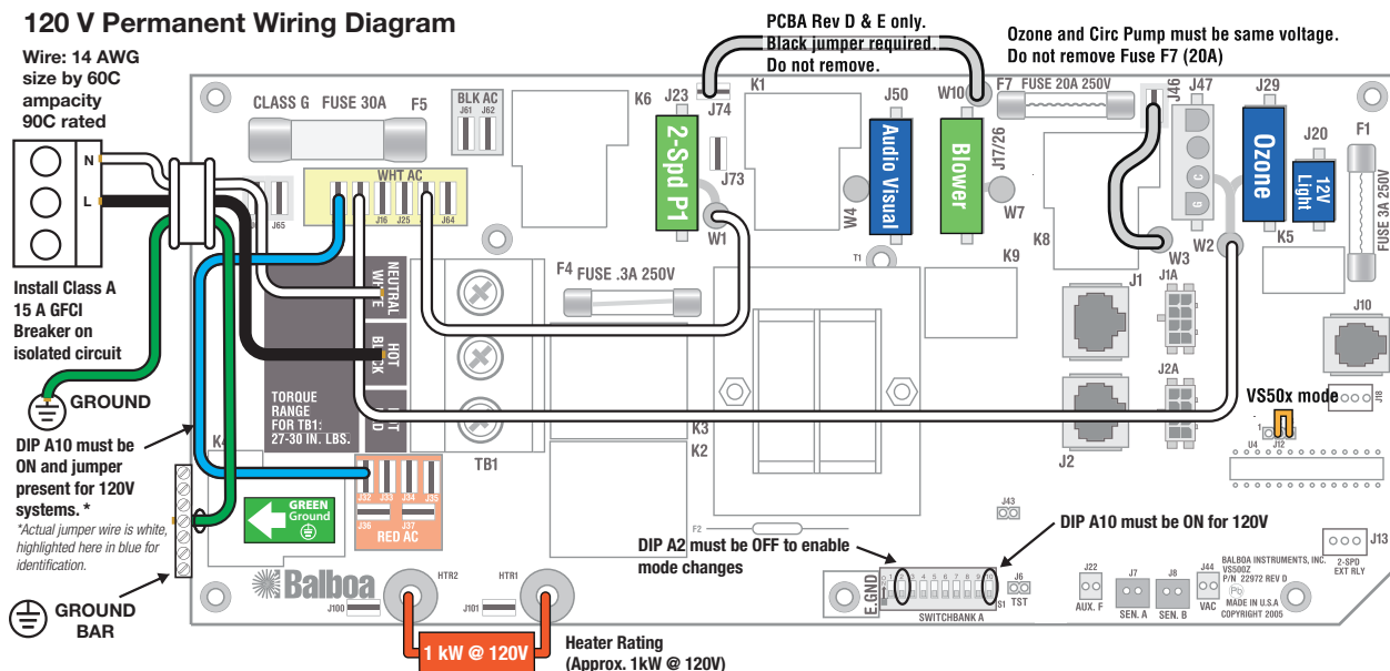
Figure A2. Wiring Diagram for 120V Permanent Wired Option 1.
