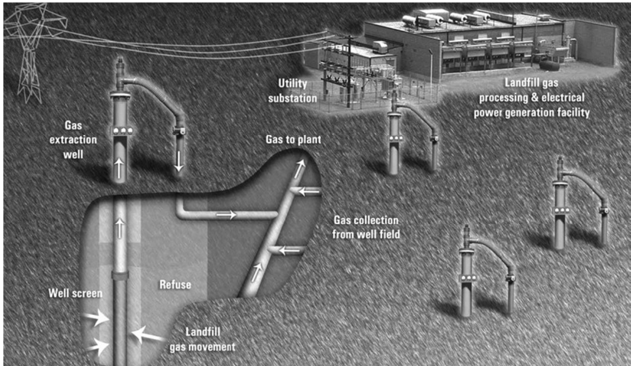
Figure 2: Typical Landfill Gas Collection and Extraction
