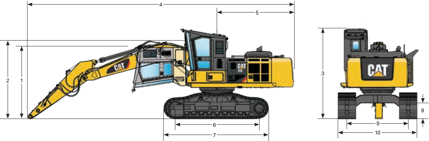
558 General Forestry - Reach with Rotate (0.457 m (18 in) riser side entry cab, boom stretched out away from the machine)
