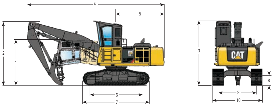
558 LL Log Loader - Under/Under (1.219 m (48 in) riser side entry cab, boom tucked towards the machine)
