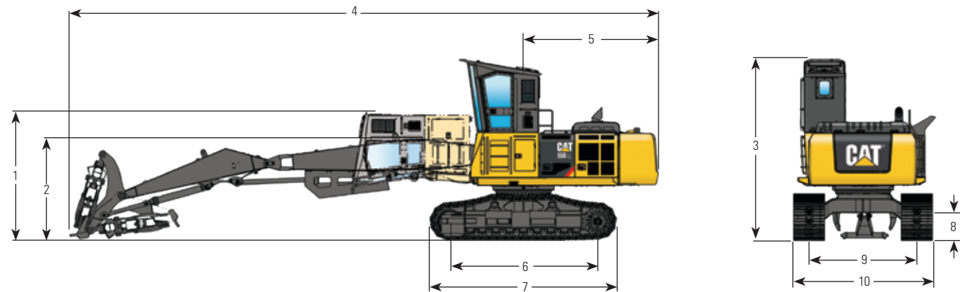
558 LL Log Loader - Under/Under (1.219 m (48 in) riser side entry cab, boom stretched out away from the machine)
