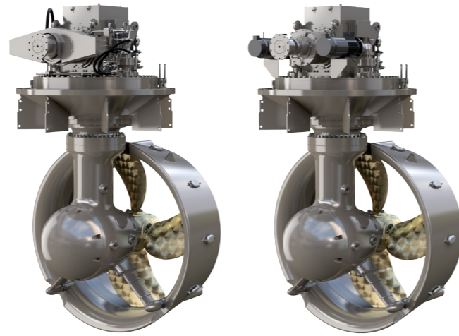
Hydraulic steering
