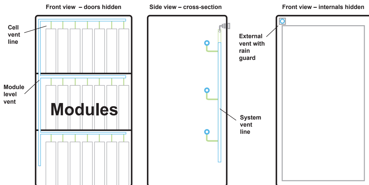
Figure 1: Cat® Energy Storage module layout
