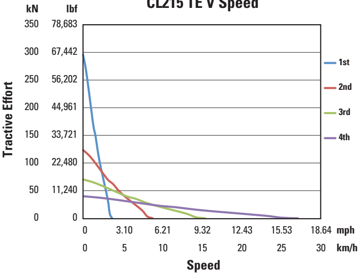
CL215 TE V Speed
