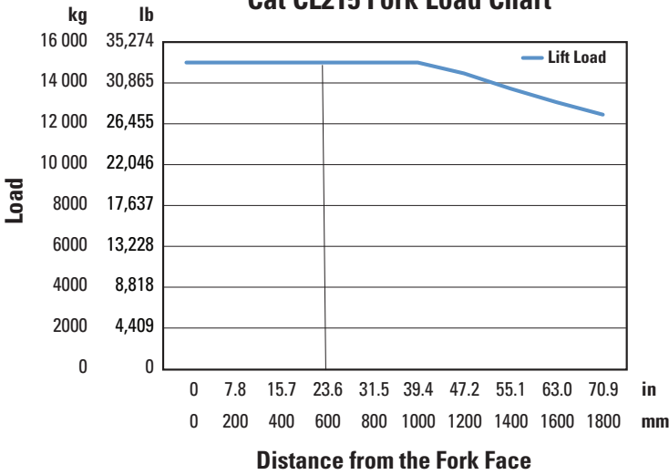
Cat CL215 Fork Load Chart
