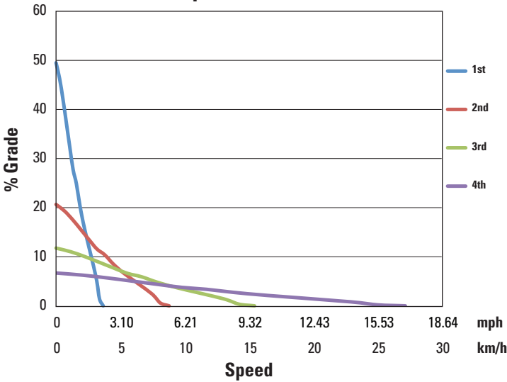
CL215 Speed V Grade Laden
