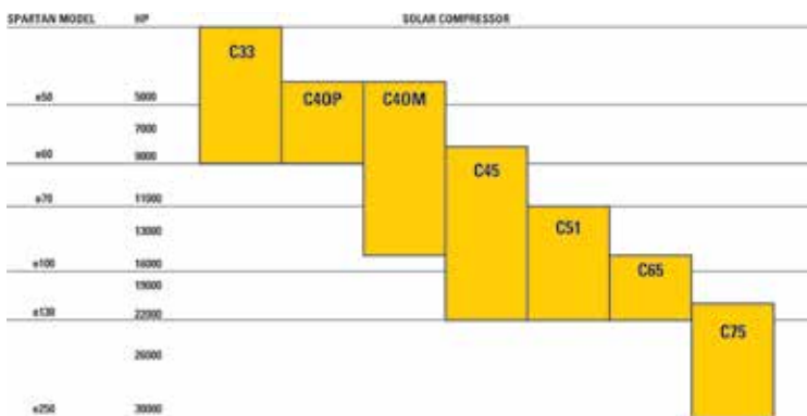
Motor Matched to Compressor Capabilities
