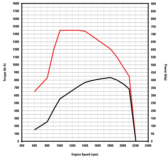
Cat CT13 – 410 bhp @ 1700 rpm
