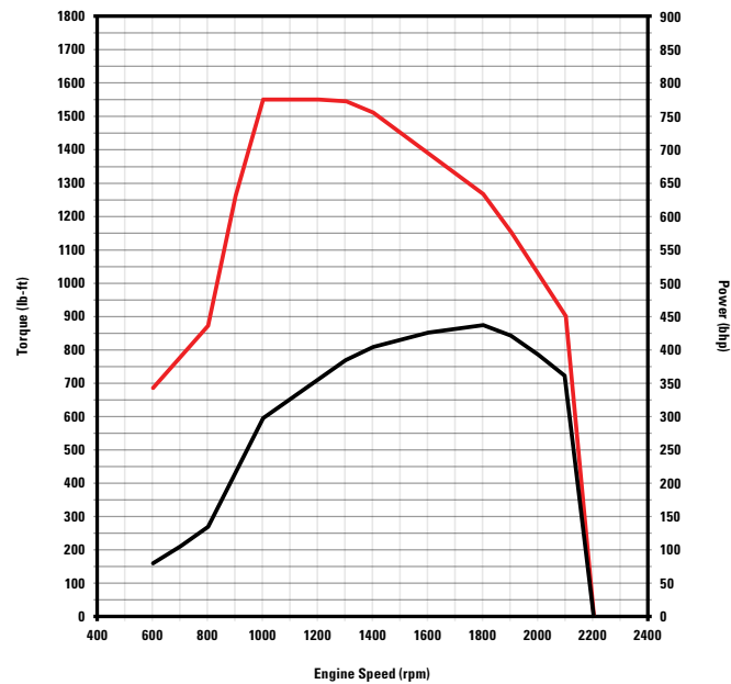
Cat CT13 – 430 bhp @ 1700 rpm
