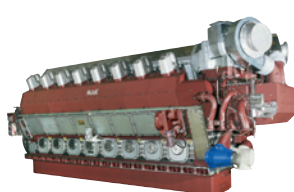
● VM 43 C 12, 16 cylinder 10,800–16,800 kW
