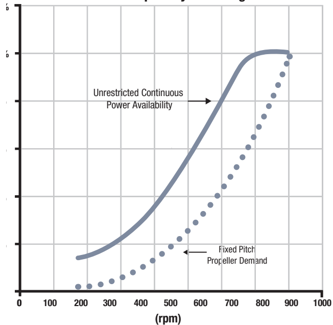
Power Capability and Margin
