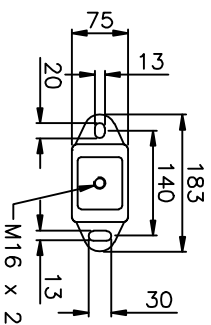
FLEXIBLE ENGINE MOUNT 'B'
