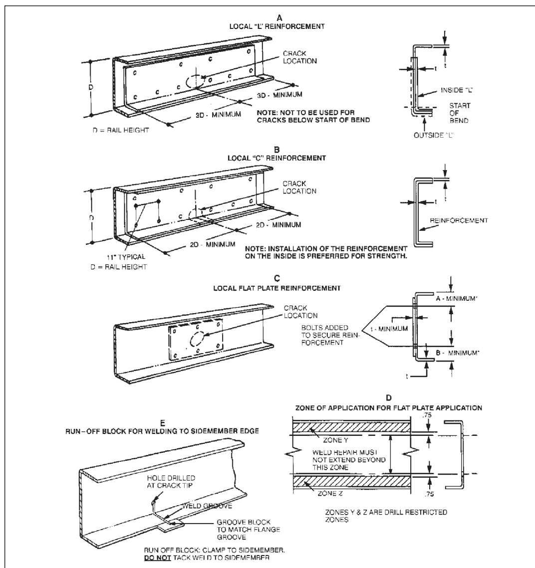
Figure 1.5 Reinforcement Application
