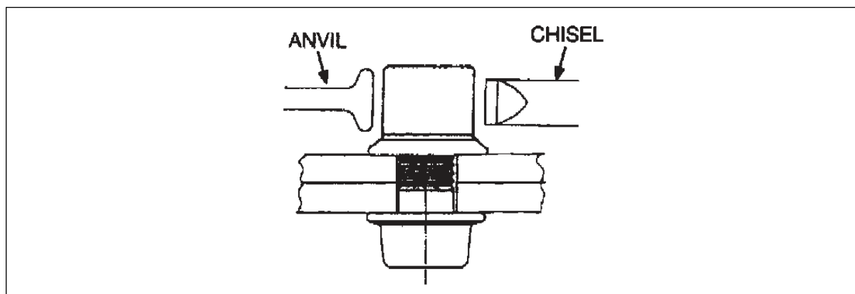
Figure 1.8 Collar Can Be Split With an Air Chisel
