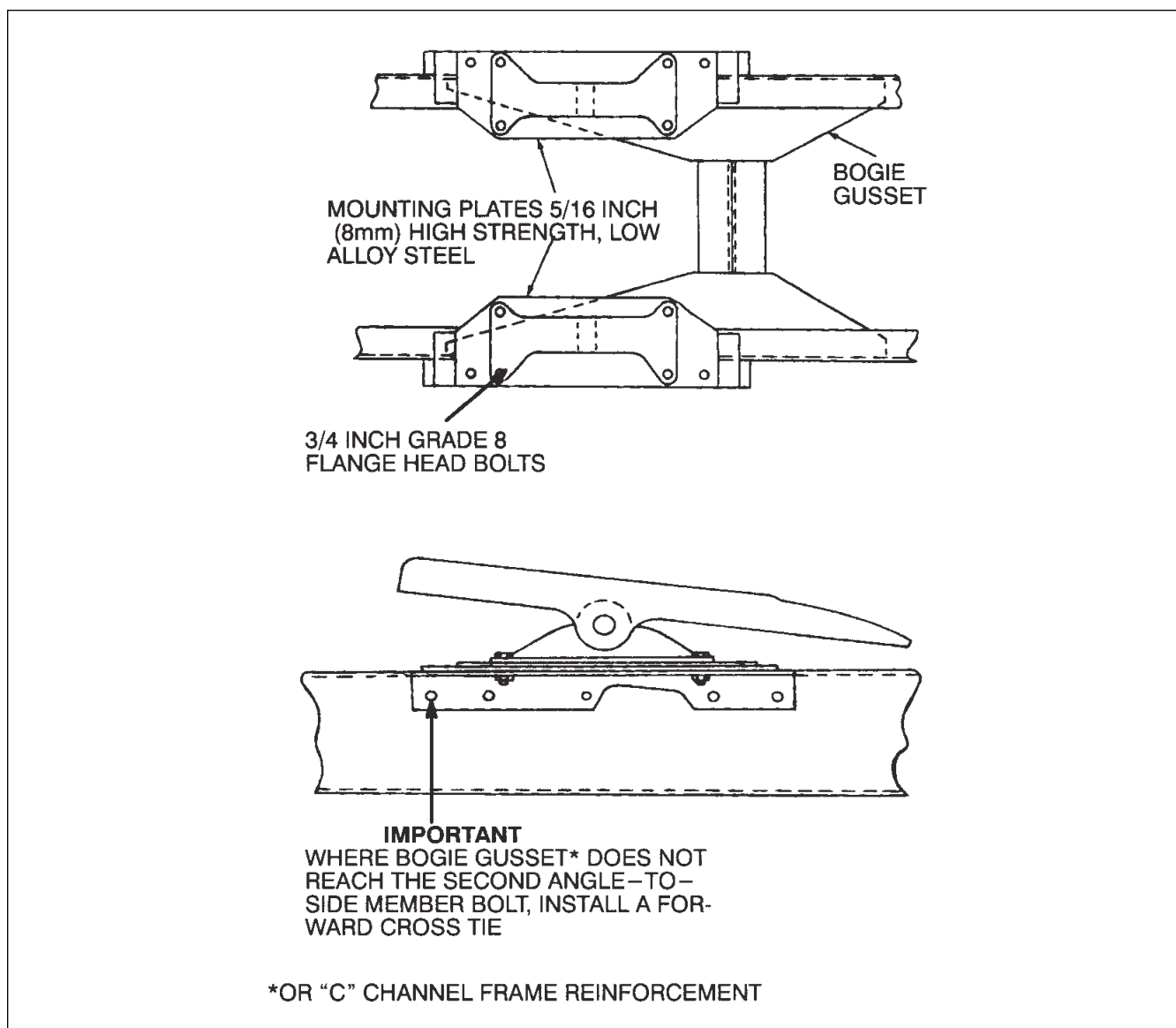
Figure 1.10 Fifth Wheel Installation Without Cross Ties (Typical)
