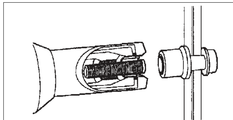
Figure 1.12 Body of Fastener Separates at Breakneck
