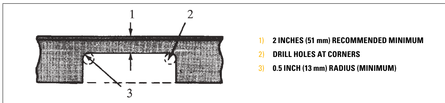
Figure 1.2 Mounting Angle Cutout
