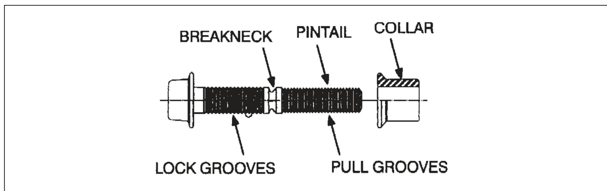
Figure 1.7 Huckbolt Fasteners
