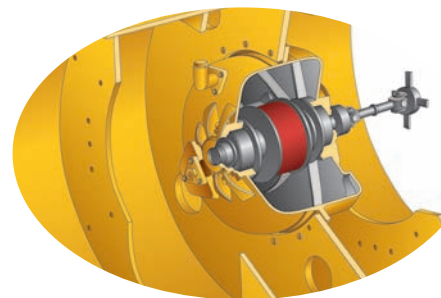
Dual Amplitude/Dual Frequency Vibratory System
